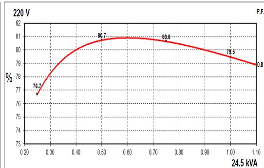
60Hz Curves
