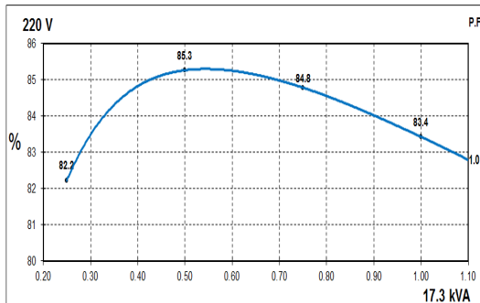
60Hz Curves
