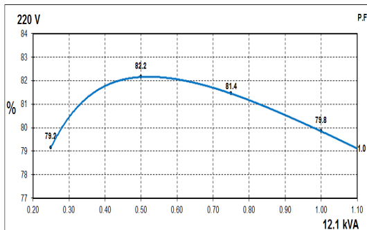
60Hz Curves
