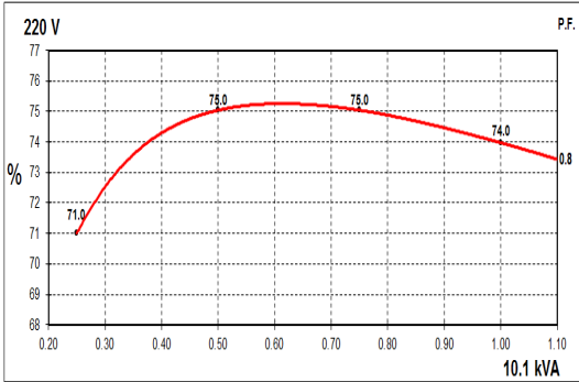
50Hz Curves
