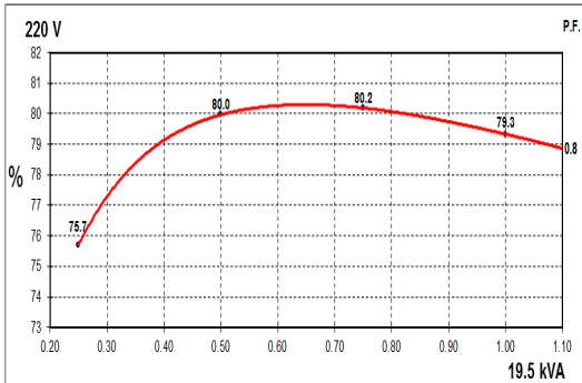
50Hz Curves
