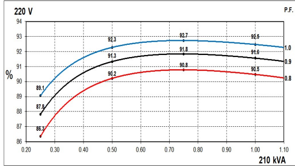
60Hz Curves
