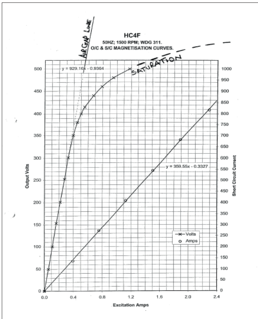
Diagram 1: Magnetisation curves:
