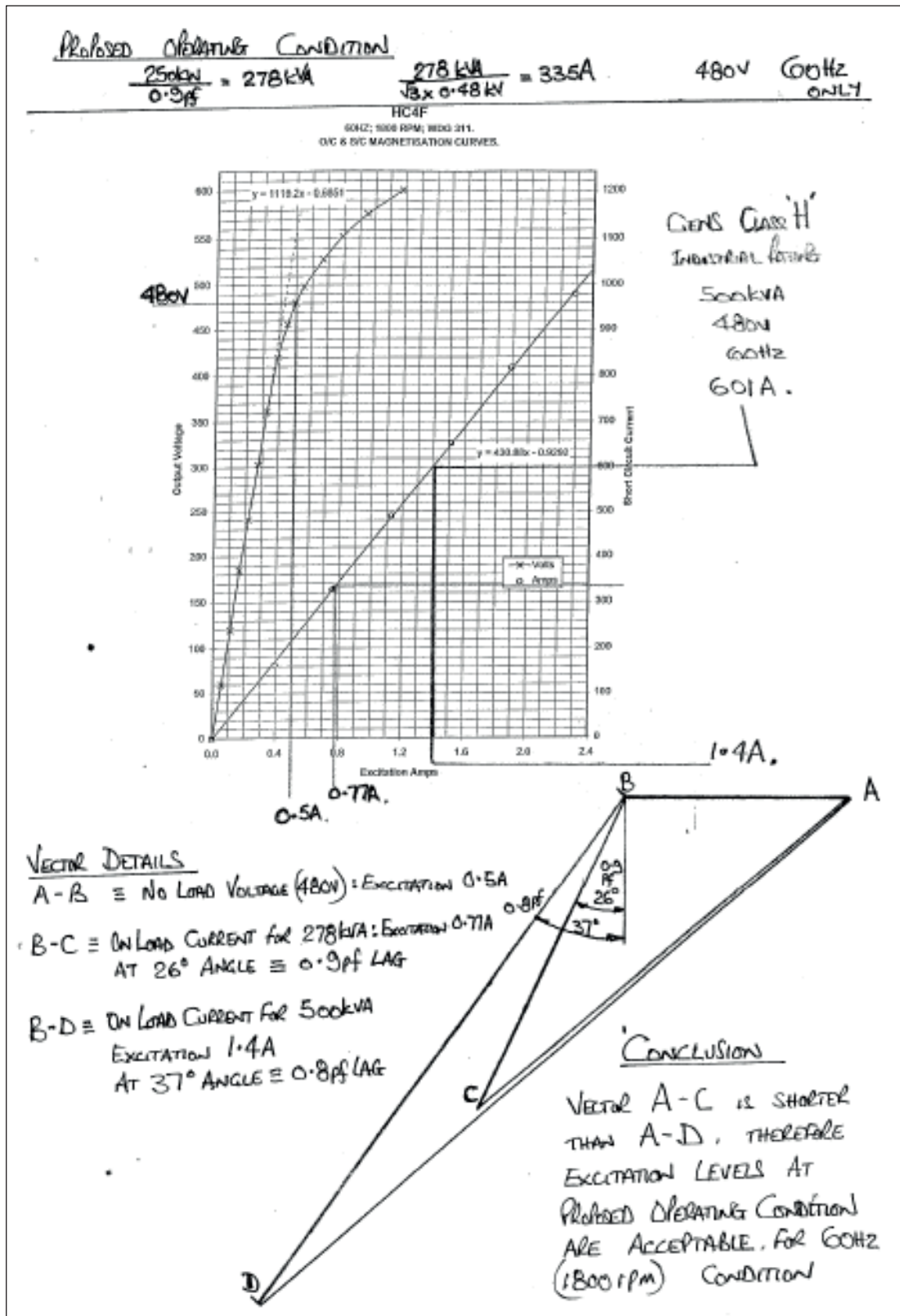
Diagram 3: Summation of excitation vectors for the no-load voltage and on-load rated current at rated power factor:
