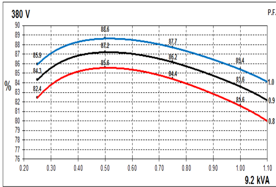
50Hz Curves
