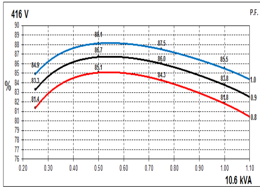
60Hz Curves
