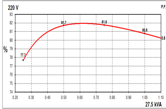
60Hz Curves
