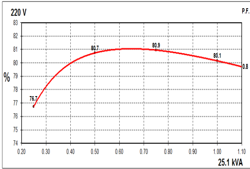
50Hz Curves
