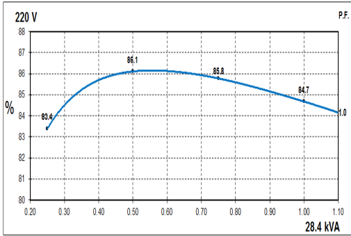
50Hz Curves
