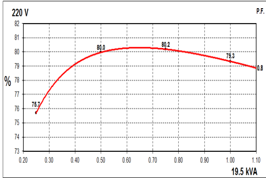
50Hz Curves
