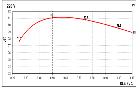
60Hz Curves
