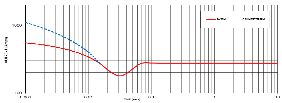
Sustained Short Circuit = 275 Amps
