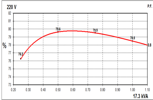
50Hz Curves
