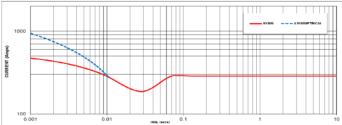
Sustained Short Circuit = 287 Amps
