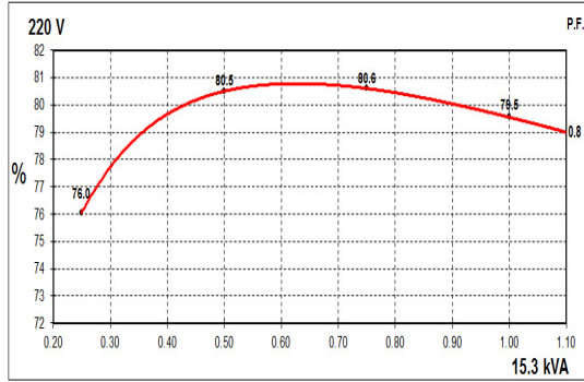
60Hz Curves
