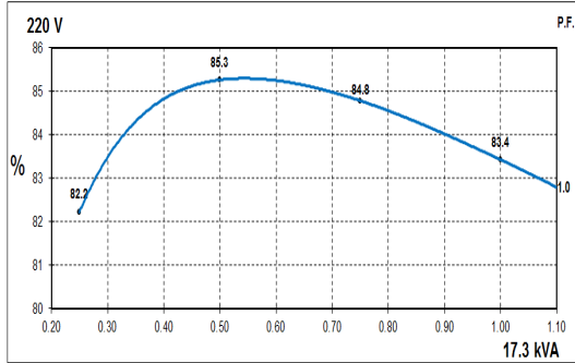
60Hz Curves
