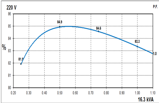
50Hz Curves
