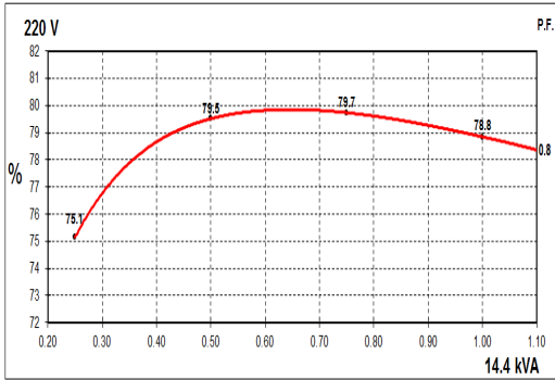
50Hz Curves
