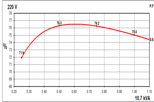
60Hz Curves
