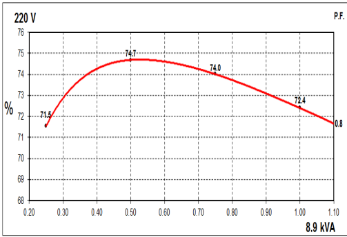
50Hz Curves
