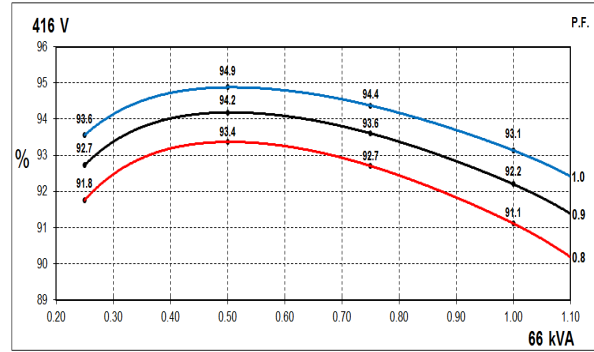
60Hz Curves
