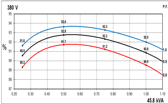
50Hz Curves
