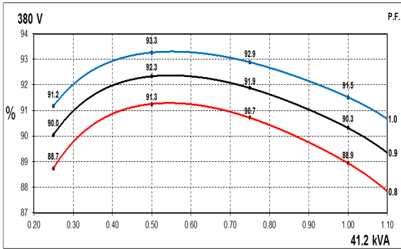
50Hz Curves
