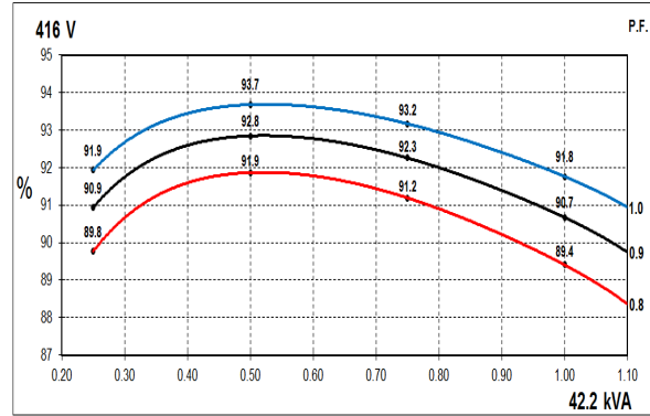
60Hz Curves
