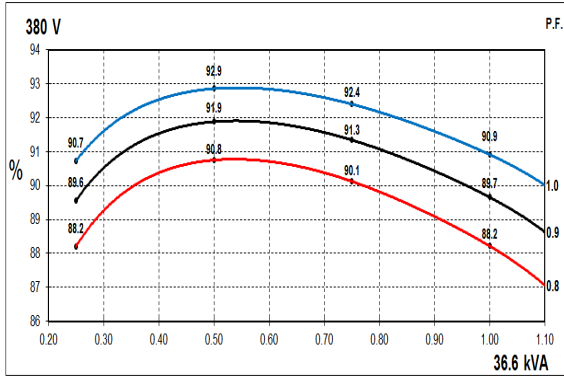
50Hz Curves
