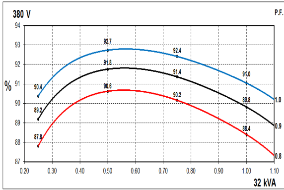
50Hz Curves
