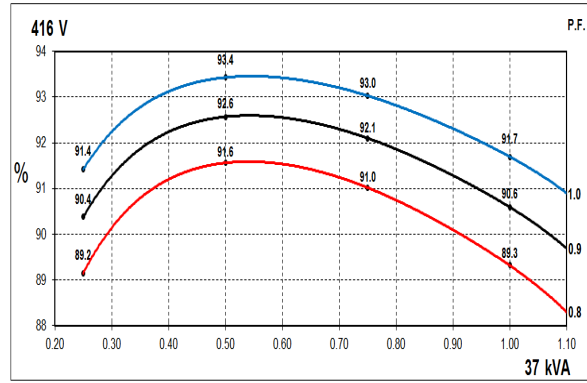
60Hz Curves
