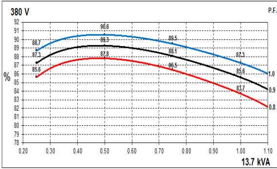
50Hz Curves
