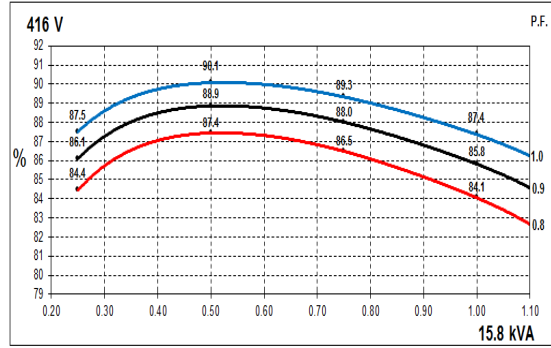
60Hz Curves
