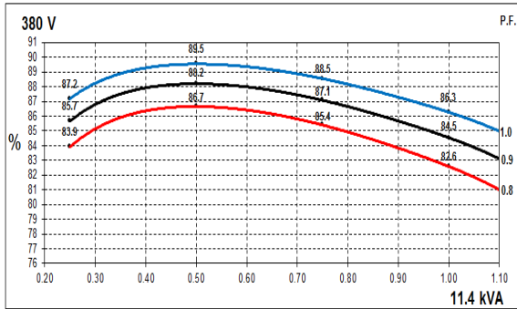
50Hz Curves
