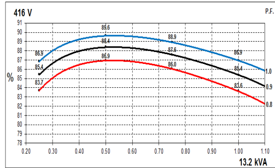
60Hz Curves
