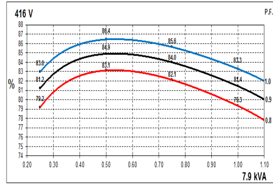
60Hz Curves
