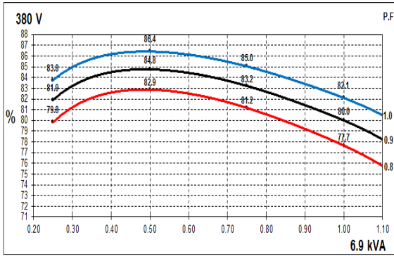
50Hz Curves
