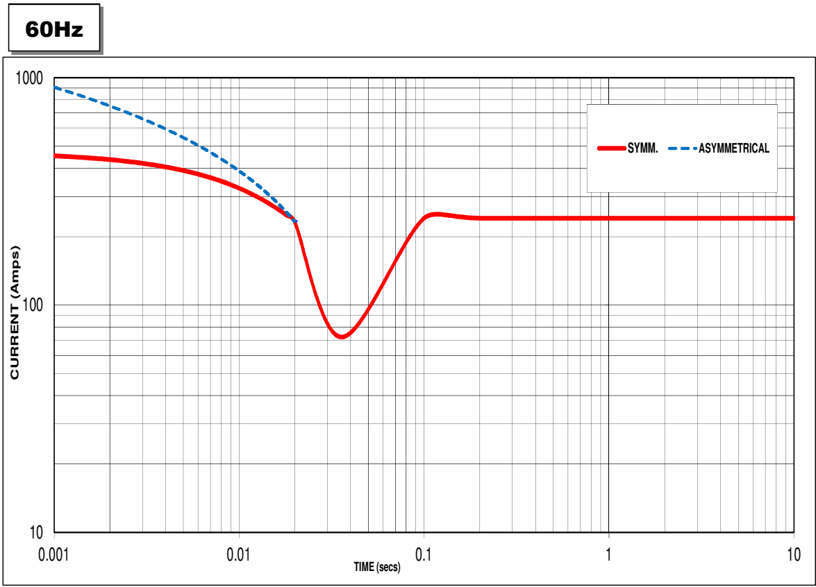
Sustained Short Circuit = 241 Amps
