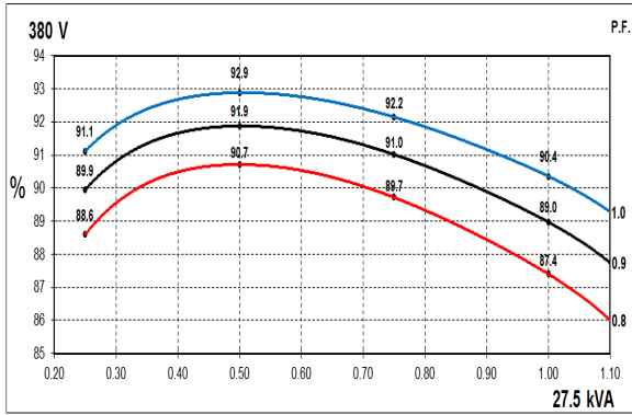
50Hz Curves
