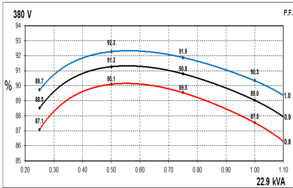
50Hz Curves
