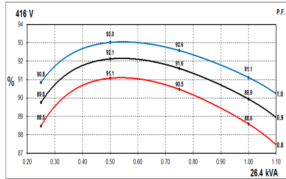
60Hz Curves
