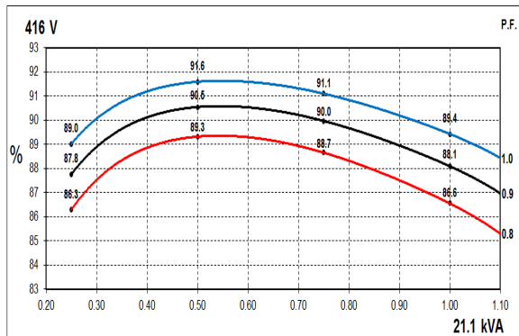
60Hz Curves
