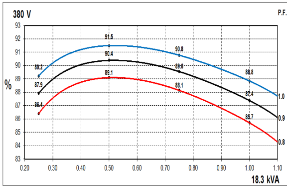
50Hz Curves
