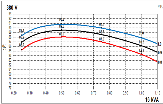
50Hz Curves
