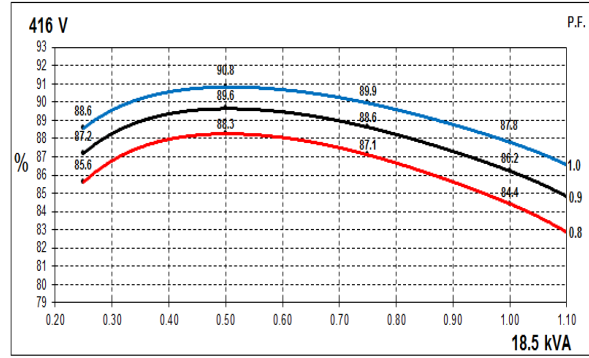
60Hz Curves
