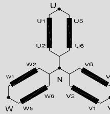
Parallel Star 3PH 4W Output Terminals (U.V.W.N.)
