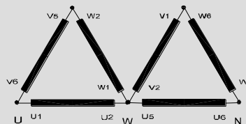
Double Delta 1Ph 3W Output Terminals (U.W.N.) (BC/UC only)
