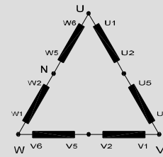
Series Delta 3Ph 4W Output Terminals (U.V.W.N.)
