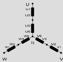
Series Star 3Ph 4W Output Terminals (U.V.W.N.)
