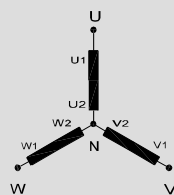
Star 3Ph 4W Output Terminals (U.V.W.N.)
