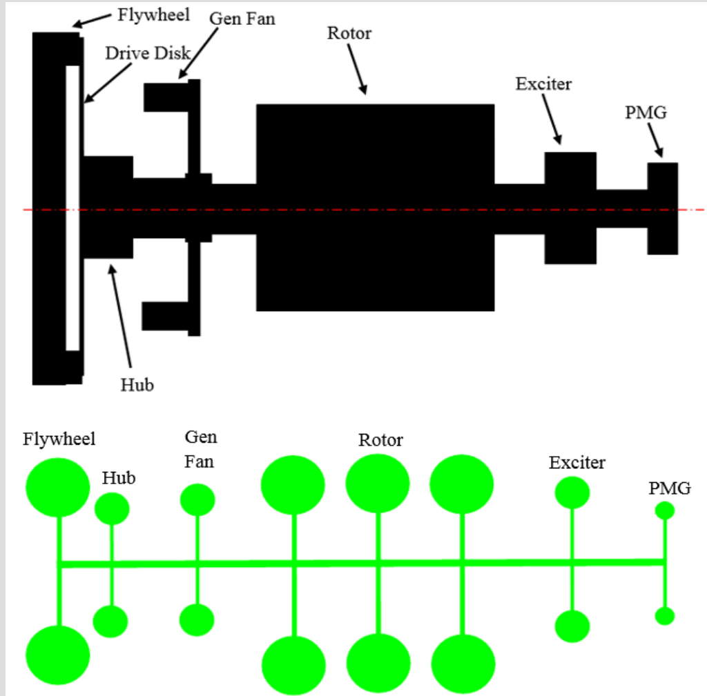
Figure 3: An equivalent linear spring/ mass system for an alternator rotor core.
