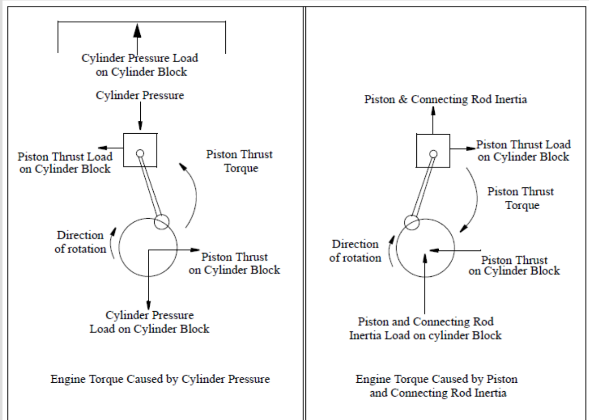
Figure 11: Movement of an internal combustion engine.
