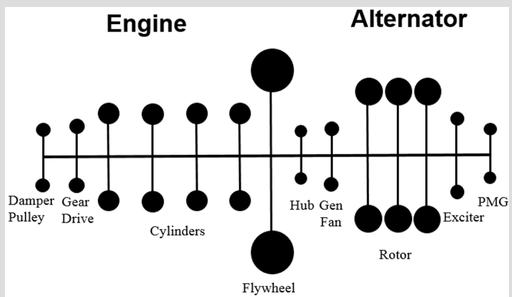
Figure 4: A complete Generating Set mass-elastic model.
