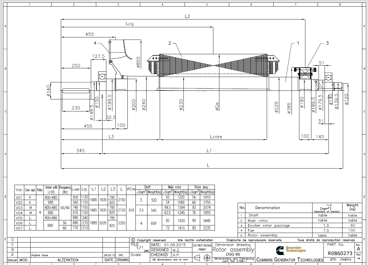
Figure 8: Typical alternator rotor drawing with shaft details.
