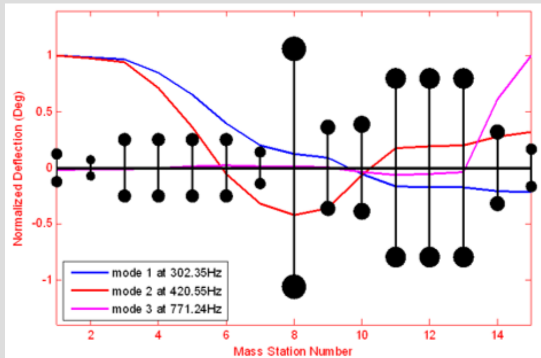
Figure 10: Typical Generating Set modal shape.
