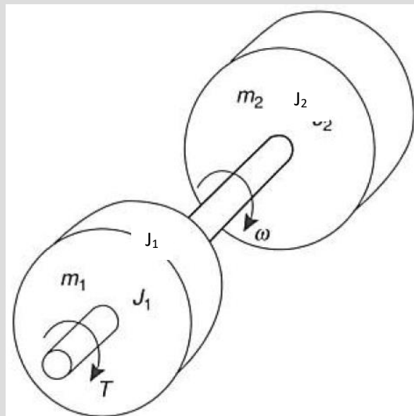
Figure 11: Two-mass torsional system.
