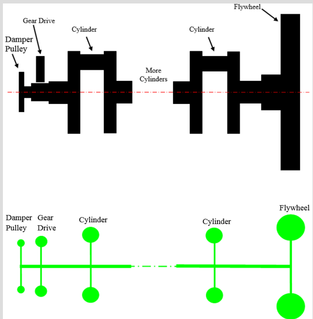
Figure 2: An equivalent linear spring/ mass system for an engine.
