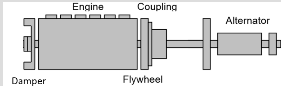
Figure 52: A complete Generating Set and areas for which data is required for TVA analysis.
