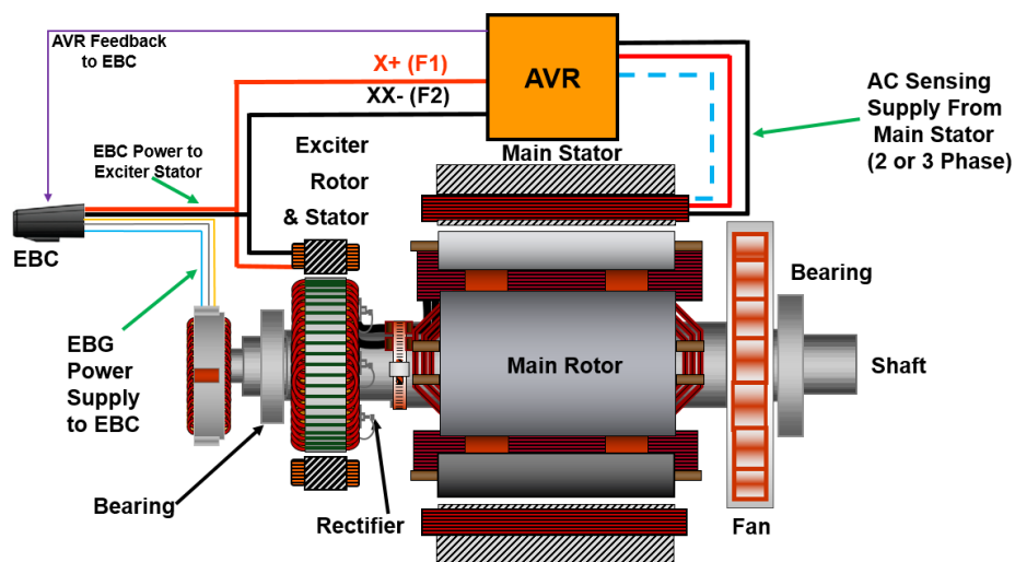
Excitation Boost System
