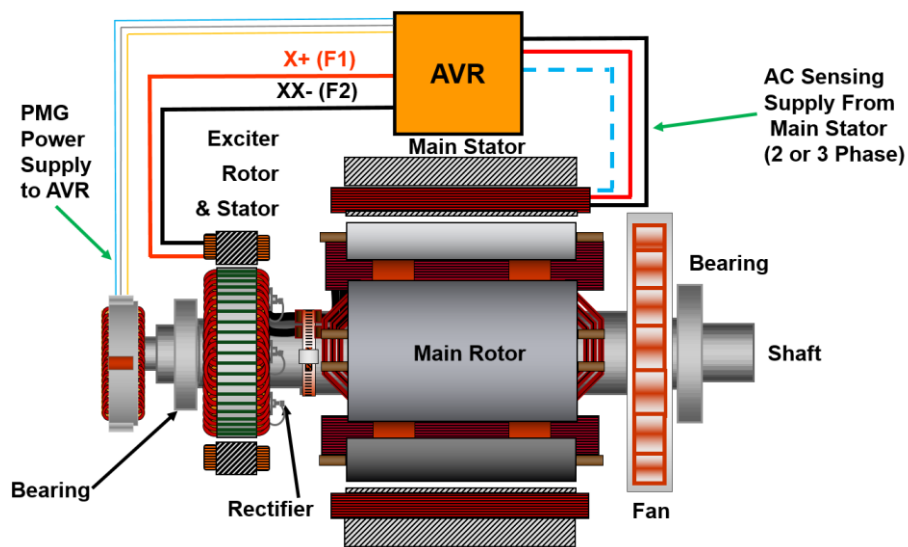
PMG Excitation System
