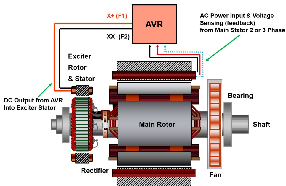
Self-Excited Alternator
