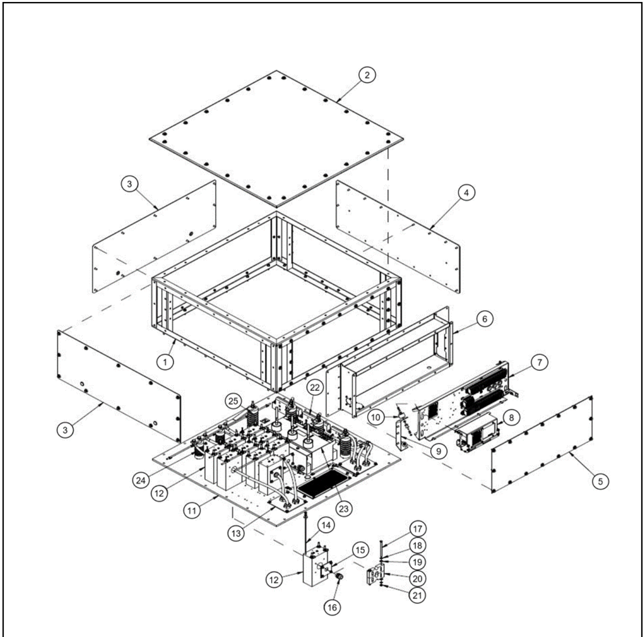
FIGURE 32. BORNIER PRINCIPAL S9 MV/HV
